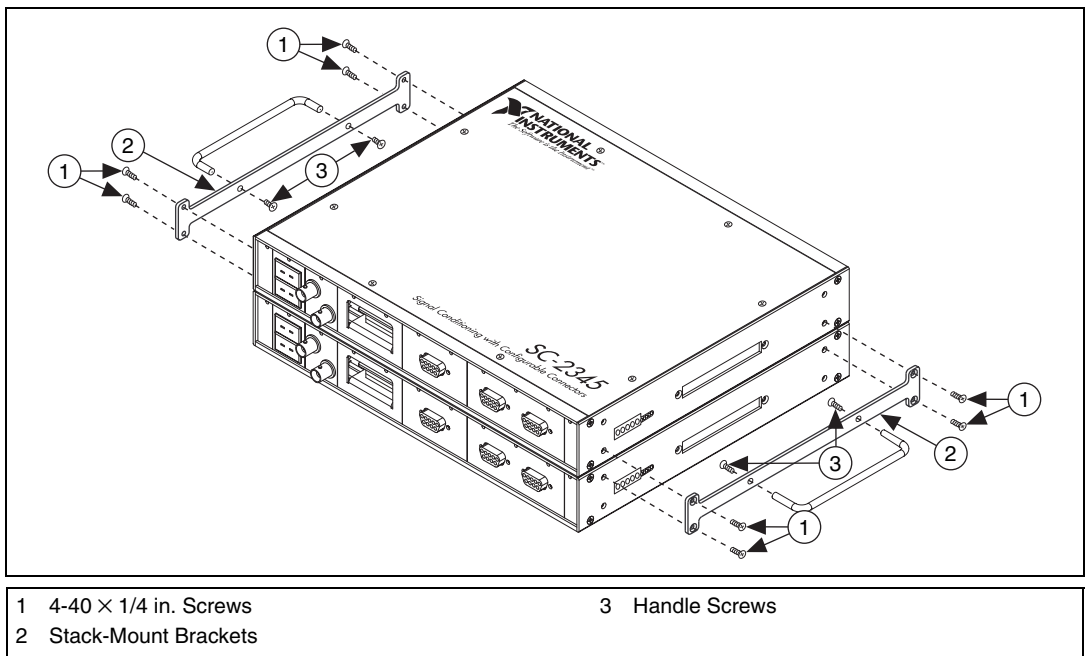
Figure 2-3. Stack-Mount Option
