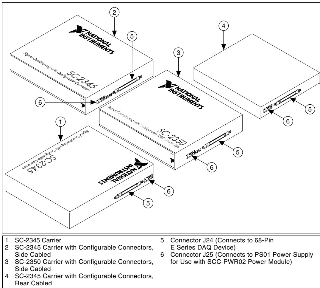
Figure 1-9. SC-2345/2350 Enclosures
