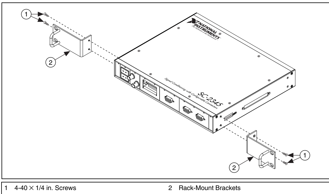
Figure 2-2. Rack-Mount Option
