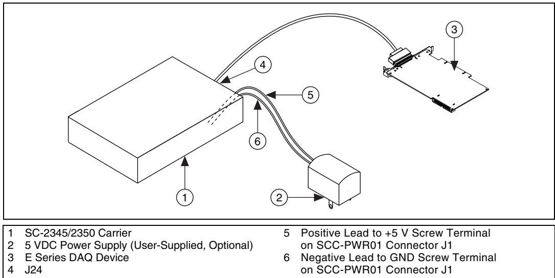
Figure 1-10. Using the SCC-PWR01
