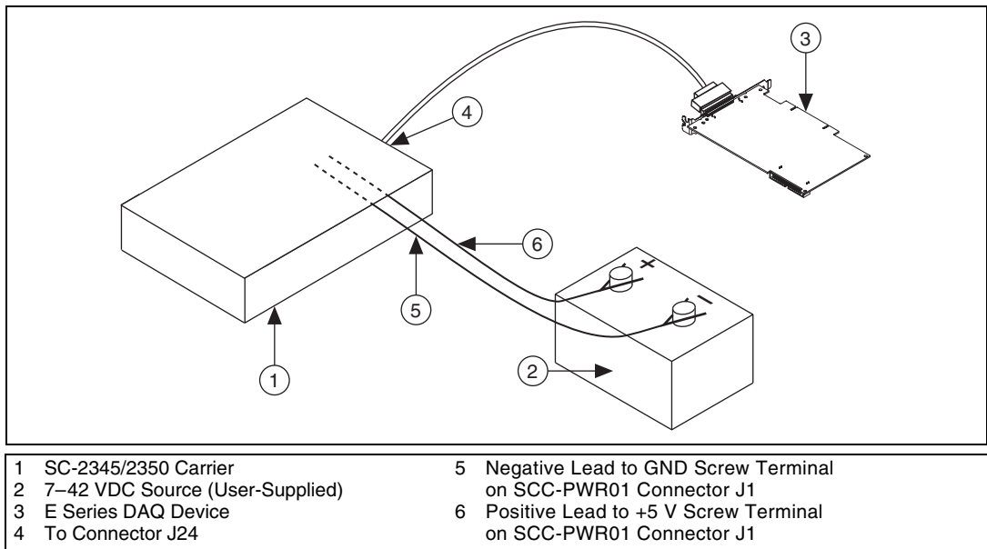
Figure 1-12. Using the SCC-PWR03
