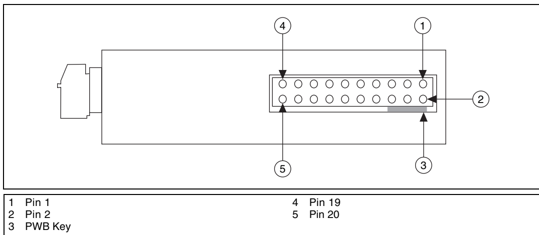
Figure B-1. SCC Module Bottom View
