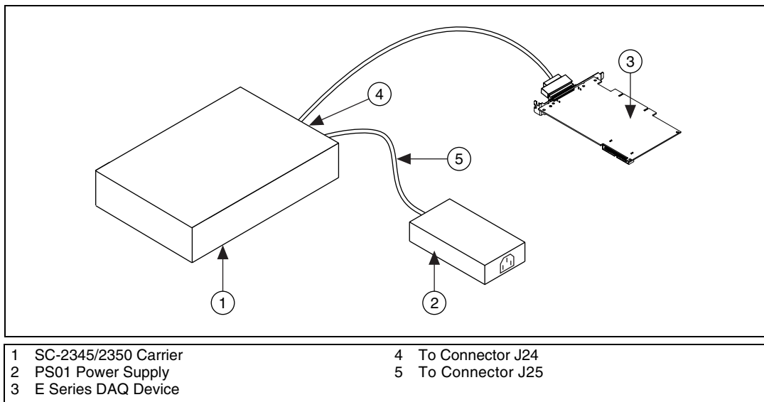
Figure 1-11. Using the SCC-PWR02
